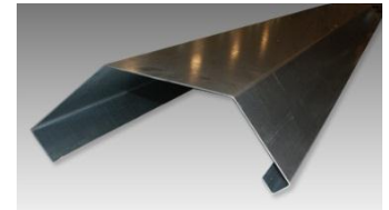
PART NO. M014001-2 DESCRIPTION: Steel Front Corner Post 111-1/8" X 14 Gauge Galvanized
